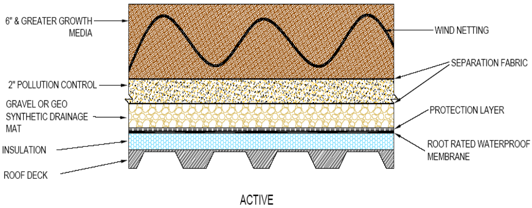
Figure 12.1b Intensive Greenroof Section (Usually Active Function)
